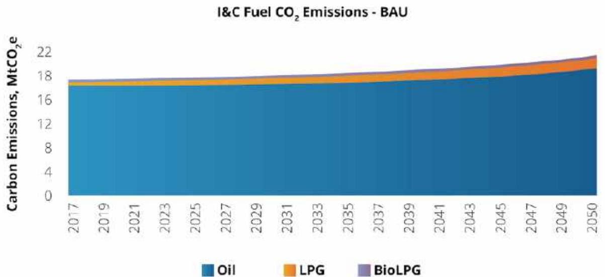
Figure 13 - Industrial & Commercial carbon emissions from oil consumption (MtCO 2 e) - business as usual scenario (Ecuity Economics)
